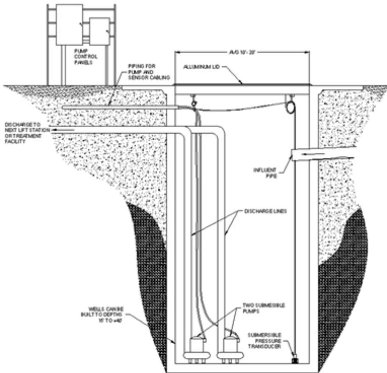
Typical Wet Well Environment
